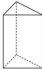
Prisma
