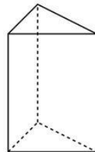
Prisma
