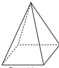
Pyramide
