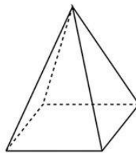
Pyramide
