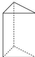
Prisma
